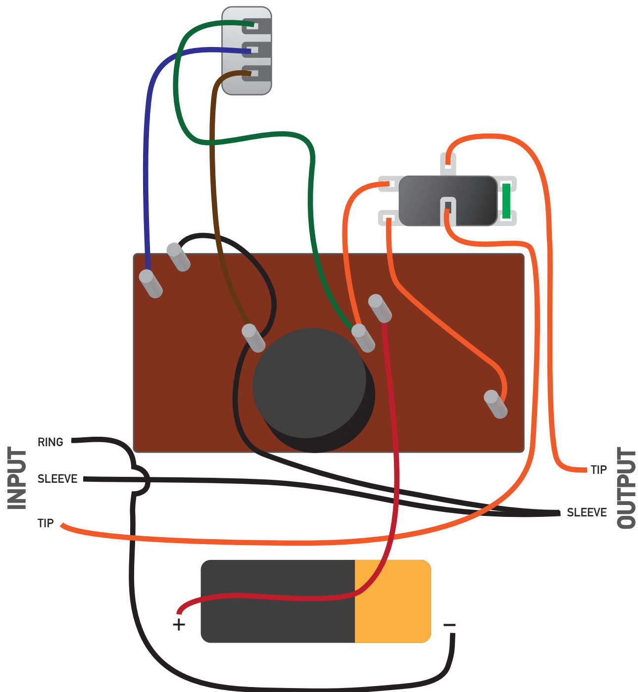
Maestro Boomerang True Bypass, Jack Swap, Volume Function Defeat
